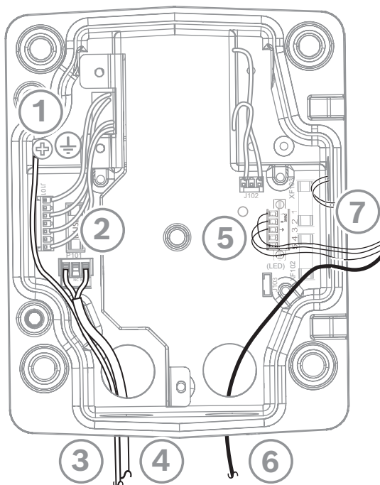
Figure 11.5: Connections for the power supply with lid (120 VAC/230 VAC models)
