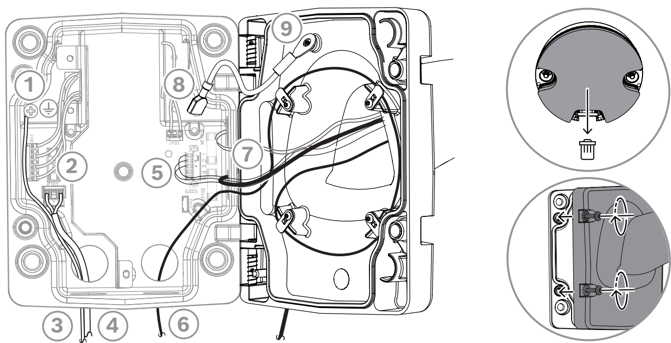
Figure 11.6: Connections for the power supply with wall arm
