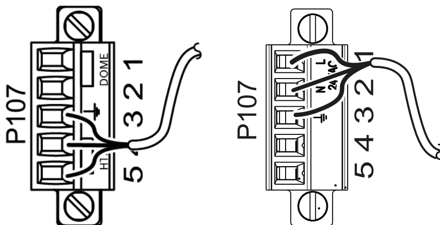
Figure 11.4: Outgoing 24 VAC connections from P107 for:
