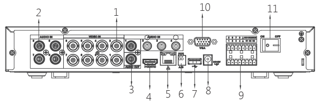
DHI-XVR5108HE-S2
